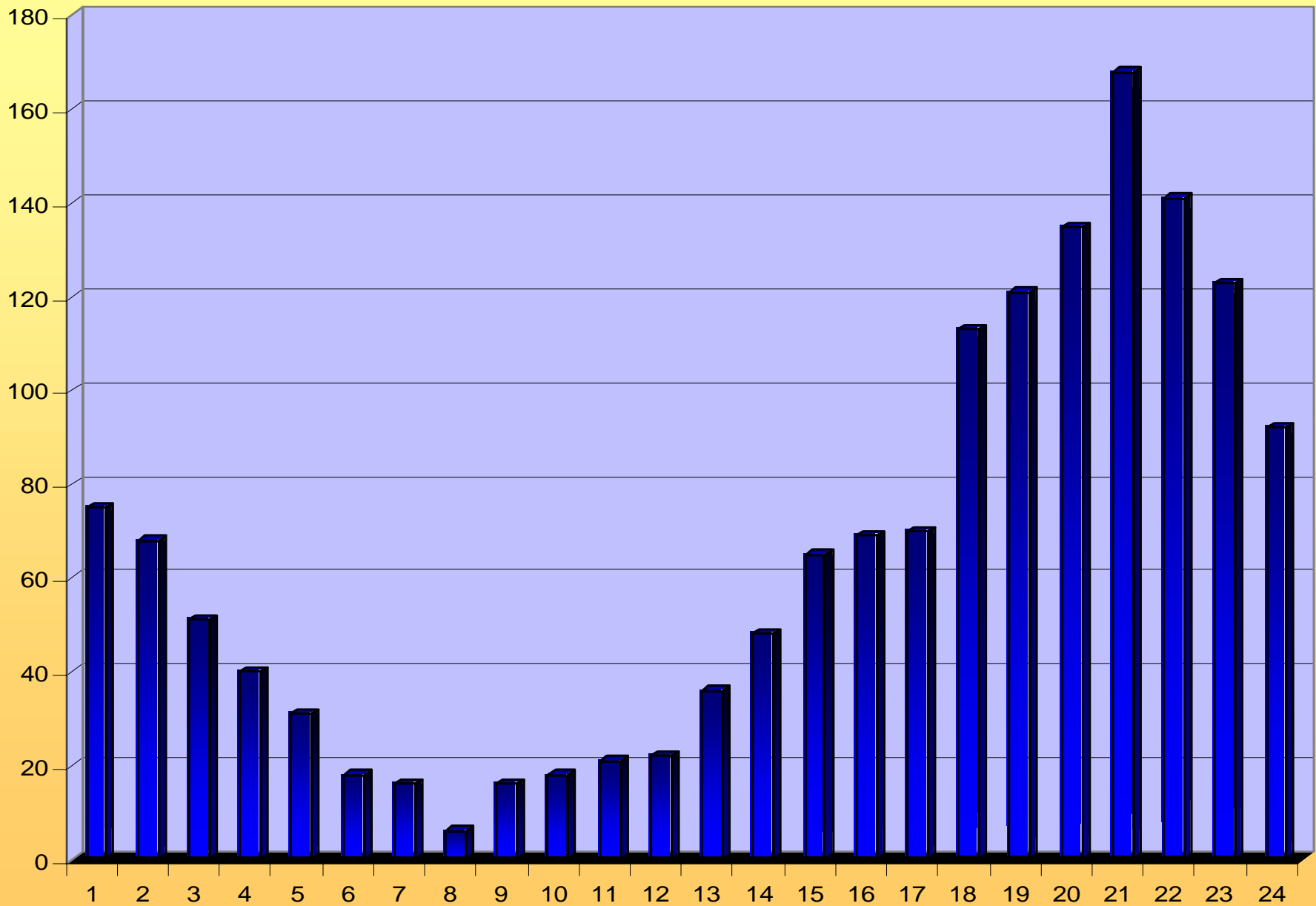
Arson Count by Hour April 04 - March 05
