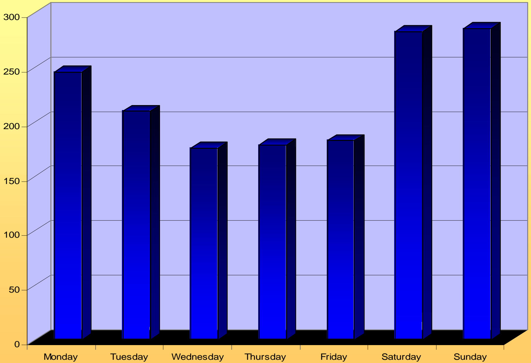
Arson by Day of Call April 04 - March 05
